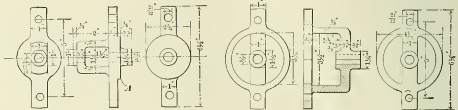
DETAILS OF A HANDY TOOL FOR AIR BRAKE WORK.
